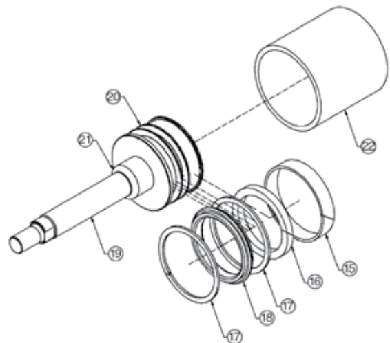
Piston/Rod Assembly
