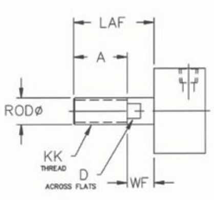
Style 1 1-1/4" Through 5" Bore Only
