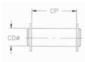
Pivot Pin for Detachable Clevis
