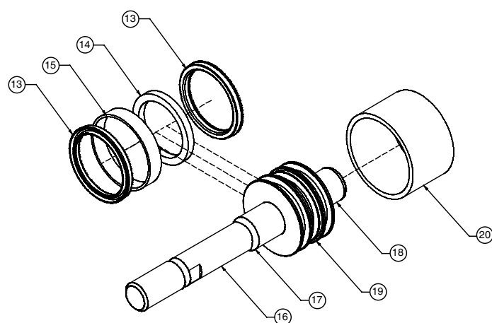
Piston/Rod Assembly
