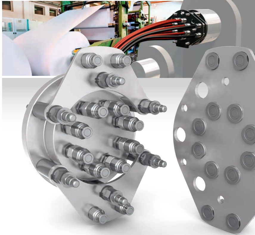
Multi-Coupling for Paper Machines Manual plate to connect 8 x Series 665 and 4 x Series 565. The couplings are made of stainless steel.
