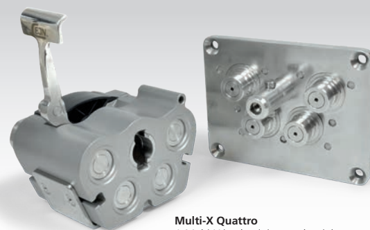
Multi-X Quattro A Multi-X in aluminium and stainless steel (AISI 316) for offshore and industrial applications.
